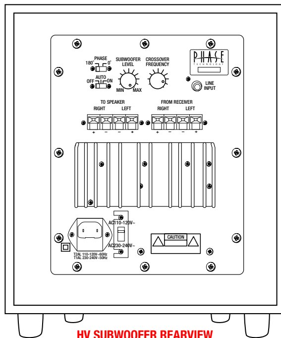
HV SUBWOOFER REARVIEW
